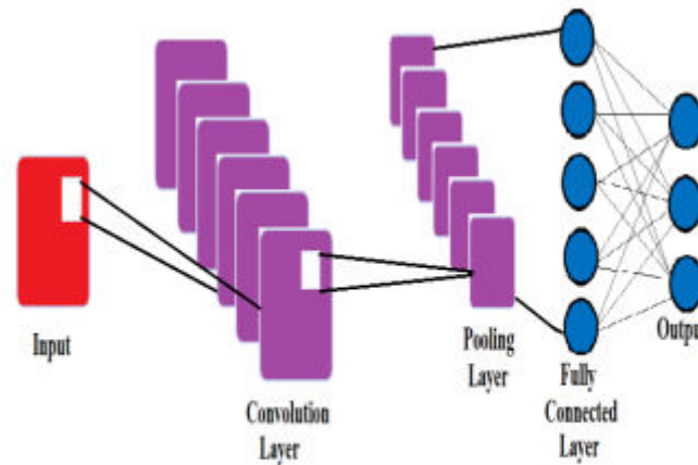
Figure 2: Cnn architecture
